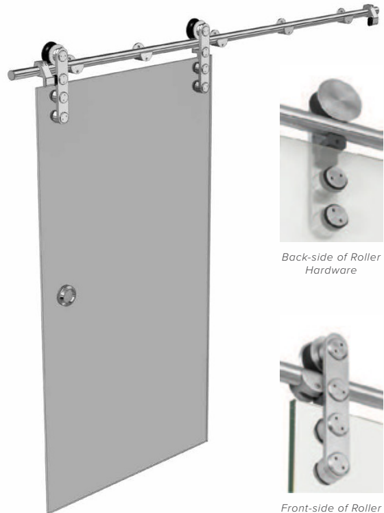
Front-side of Roller Hardware
