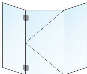
135° Neo-Angle Unit (135° glass-to-glass, side mount hinges)
