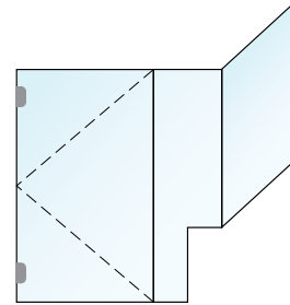
Door with Notched Fixed Panel & 90° Return on Knee Wall (side mount hinges)
